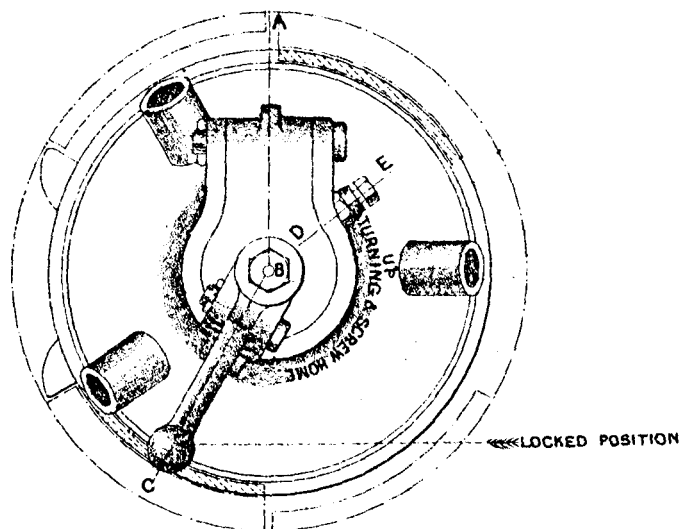
SECTION THRO' D.E. BREECH RING LOCKED
