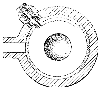
SECTION THRO' D.E. SHEWING SAFETY BOLT & BREECH RING
