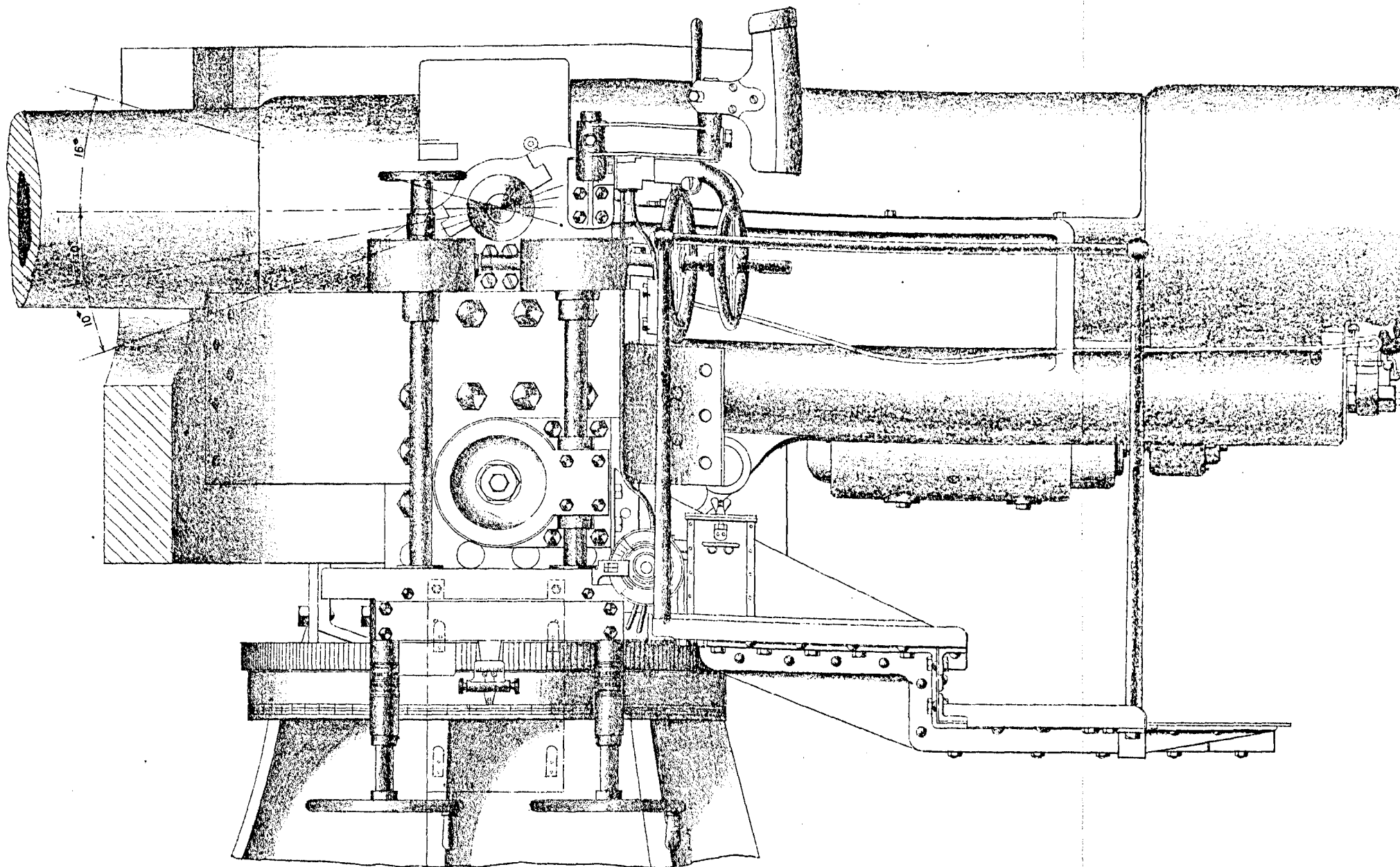
SIDE ELEVATION.
