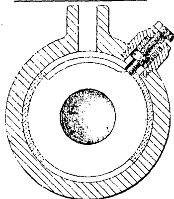
SECTION THRO' D.E. BREECH RING LOCKED
