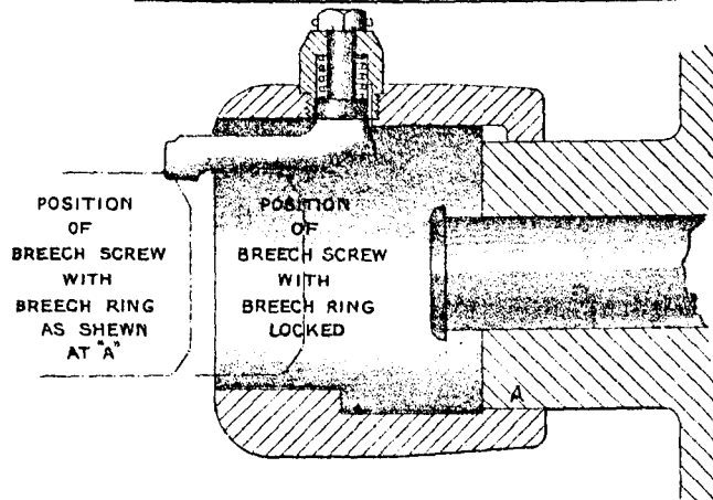
SECTION THRO' D.E. SHEWING SAFETY BOLT & BREECH RING
